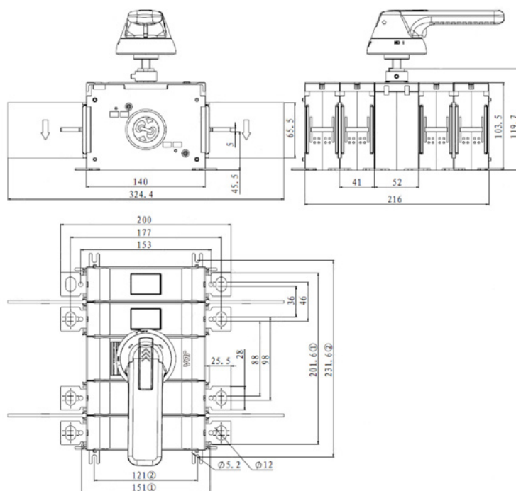
Standard Operation (Mechanism Centered) Outline Installation Drawing
