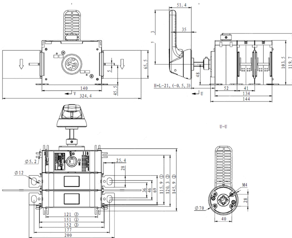
Side operation outline installation drawing
